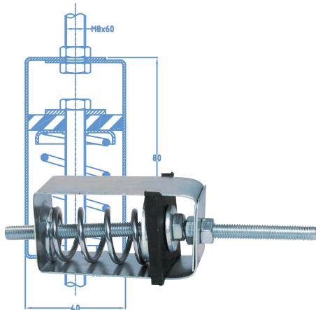
SUSTAINERS / HANGER / SUSPENTES SCHALLSCHUTZ-DECKENELEMENTE
