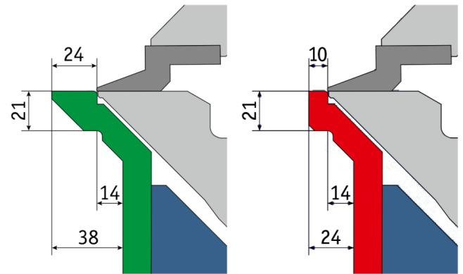
2 insert rails for bending beam as standard (10 mm and 24 mm)
